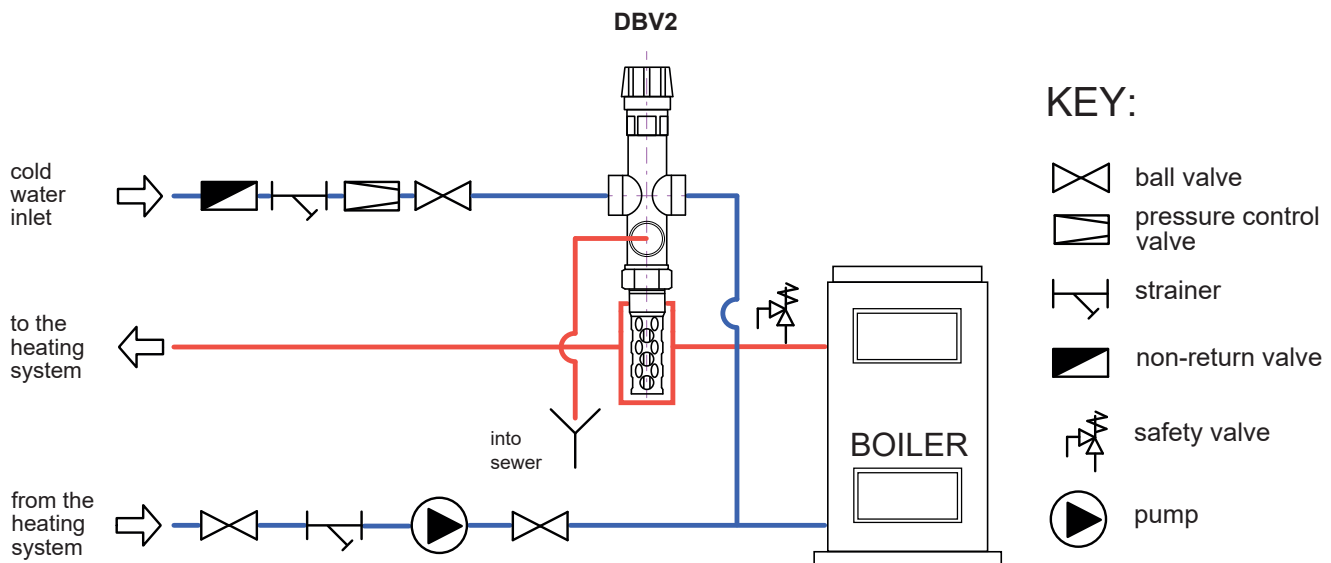
Fig. 3: Piping diagram for DBV2
