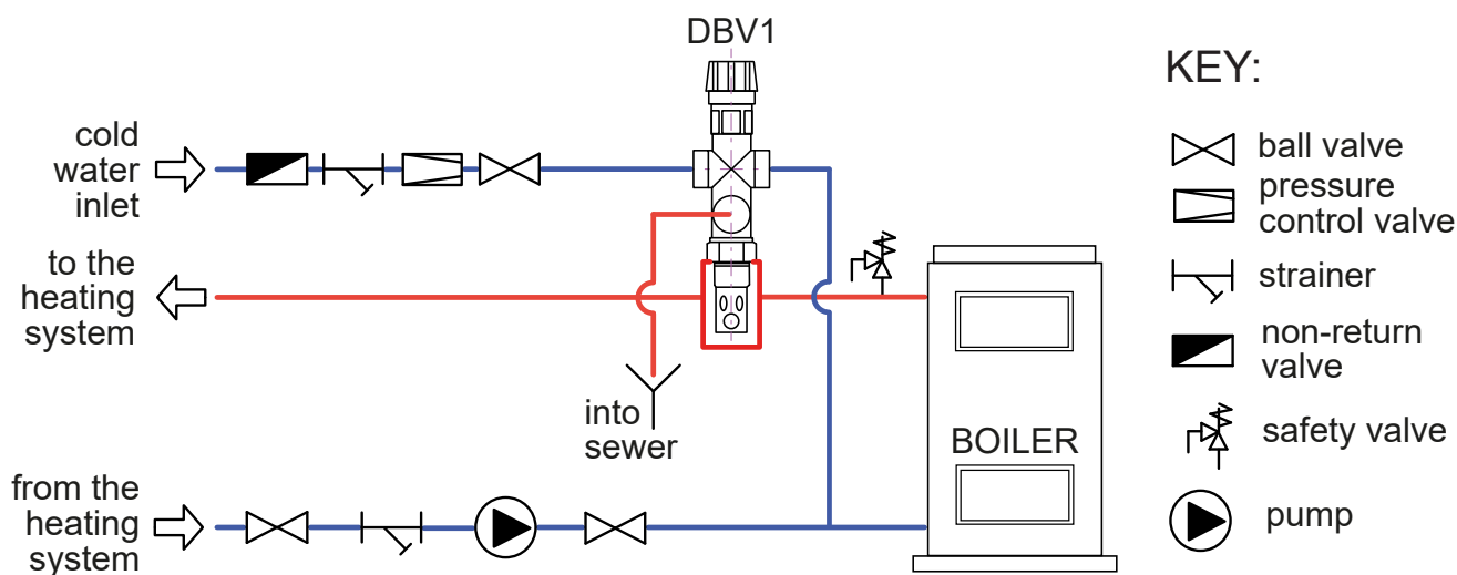
Pic. 3: Piping diagram for DBV1
