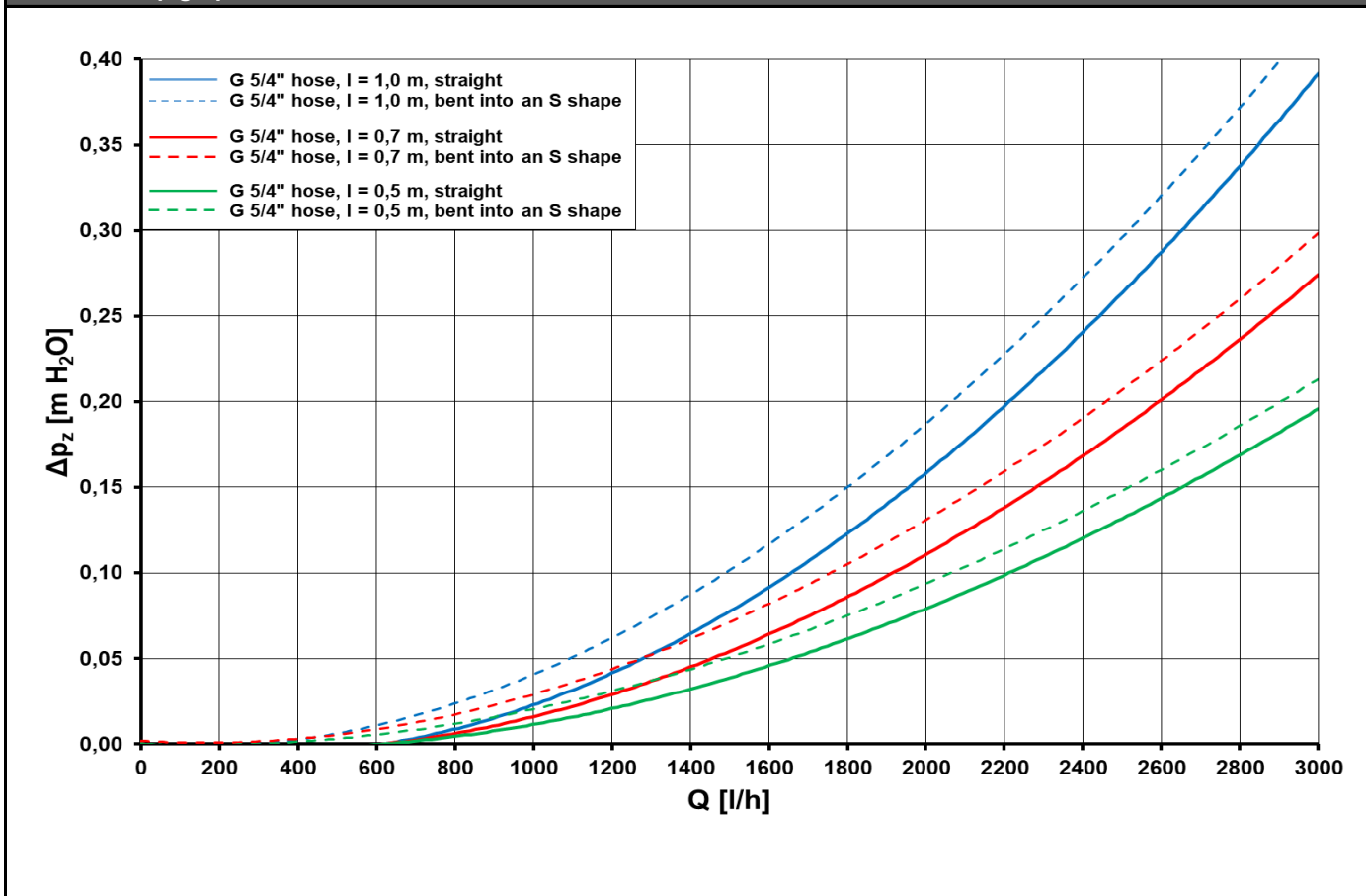
Pressure drop graph for a G 5/4" hose
